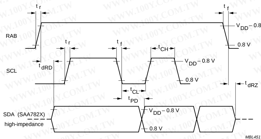
Fig.36 4-wire microcontroller timing; read mode (Q-channel subcode and decoder status information).
