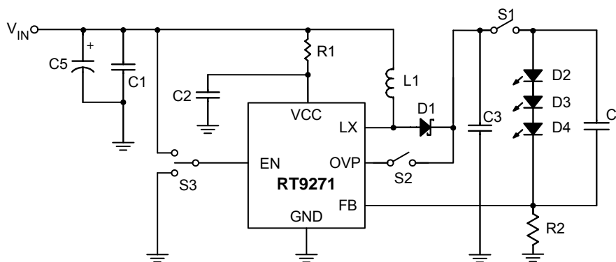
EVB Circuit
