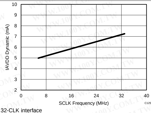
Figure 39. Analog Supply Current vs SCLK Frequency
