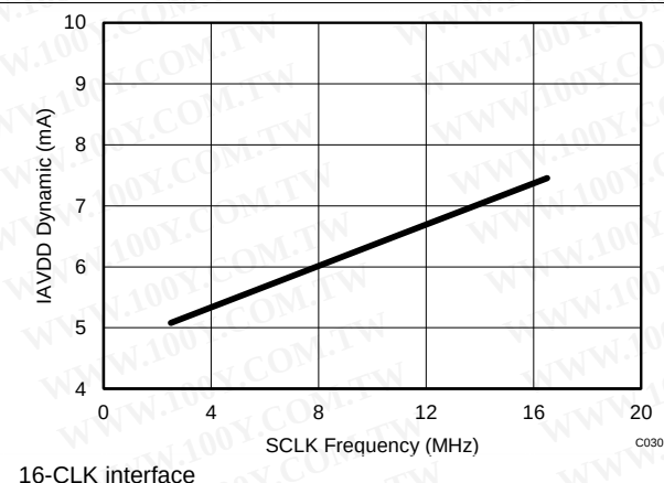
Figure 38. Analog Supply Current vs SCLK Frequency
