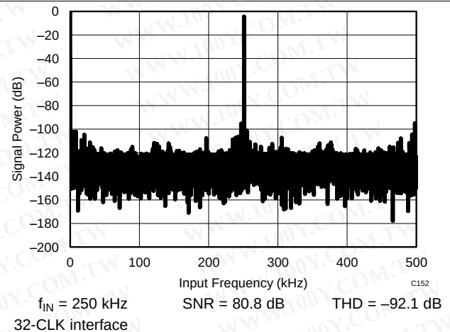
Figure 27. Typical FFT
