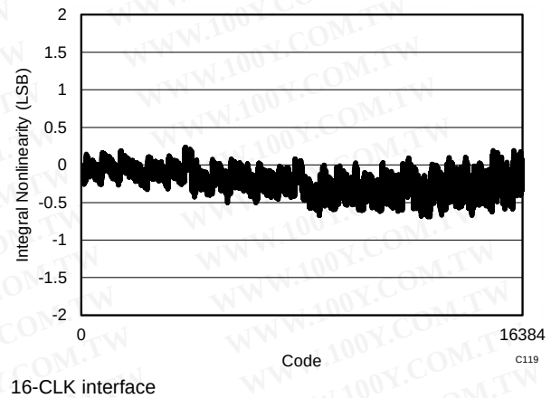
Figure 45. Typical INL
