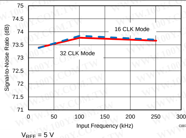
Figure 60. SNR vs Input Frequency
