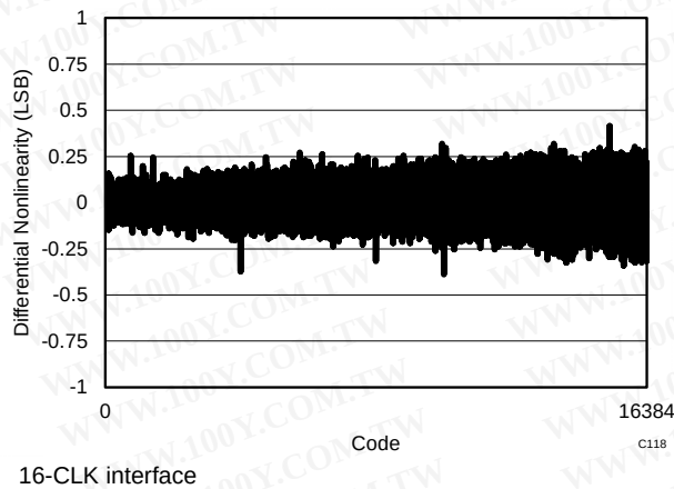
Figure 44. Typical DNL
