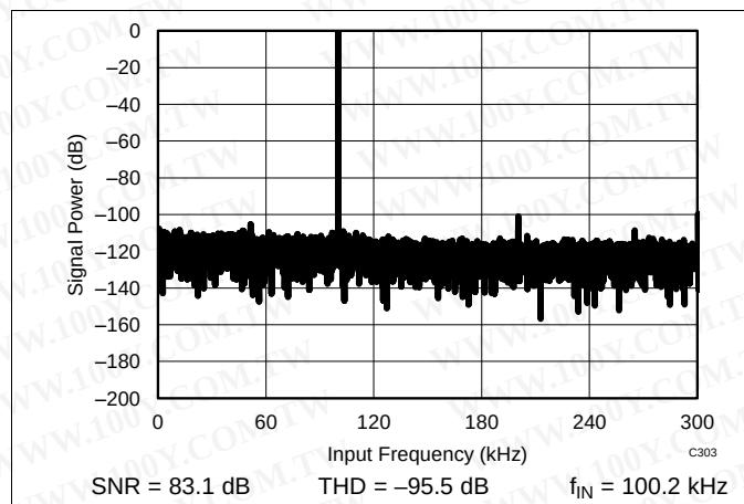
Figure 111. ADS8353 in 32-CLK Interface Mode
