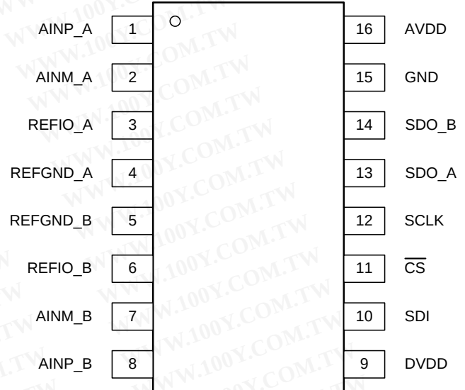
PW Package TSSOP-16 (Top View)
