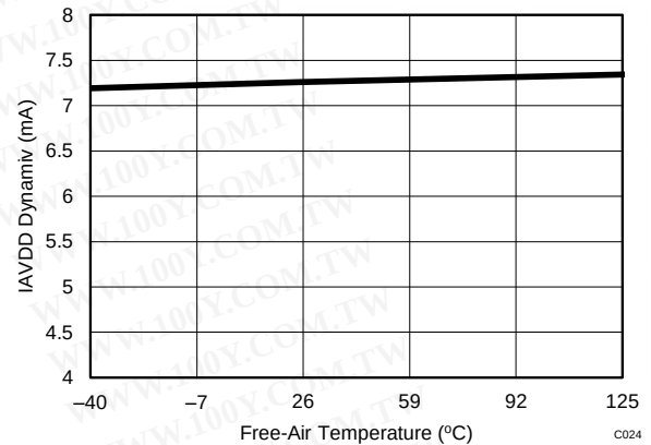
Figure 65. Analog Supply Current vs Temperature
