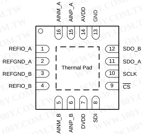
RTE Package WQFN-16 (Top View)
