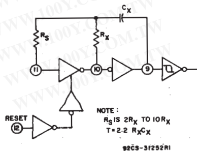
Fig. 12 - Typical RC circuit.
