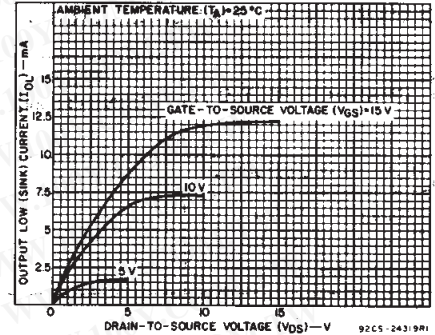
Fig. 4 - Minimum n-channel output low (sink) current characteristics.
