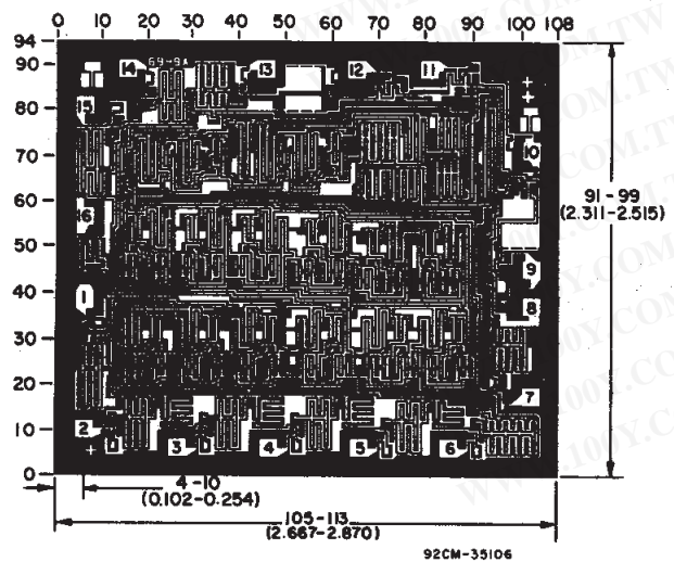
Chip dimensions and pad layout for CD4060B
