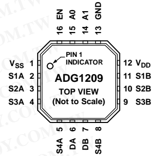
Figure 6. ADG1209 Pin Configurations (LFCSP_VQ), Exposed Pad Tied to Substrate, V SS
