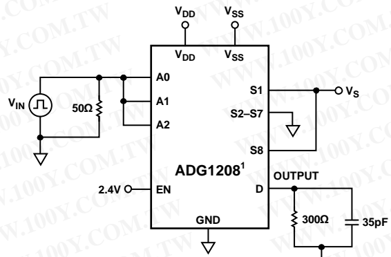
Figure 33. Break-Before-Make Delay, t_{\text{BBM}}
