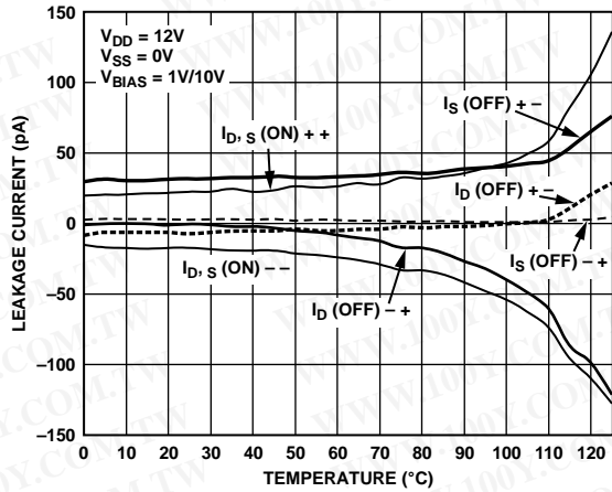
Figure 13. ADG1208 Leakage Currents as a Function of Temperature, Single Supply
