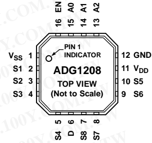
Figure 4. ADG1208 Pin Configuration (LFCSP_VQ), Exposed Pad Tied to Substrate, V SS
