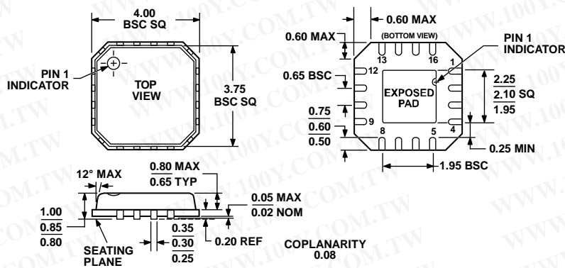
Figure 41. 16-Lead Lead Frame Chip Scale Package [LFCSP_VQ]
