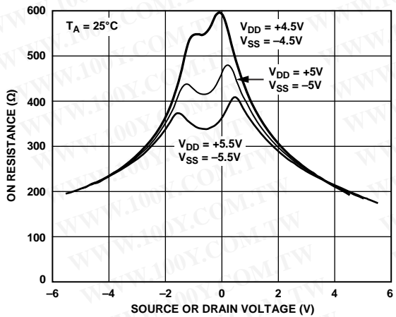
Figure 8. On Resistance as a Function of V_D ( V_S ) for Dual Supply
