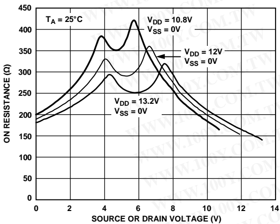
Figure 9. On Resistance as a Function of V_D ( V_S ) for Single Supply
