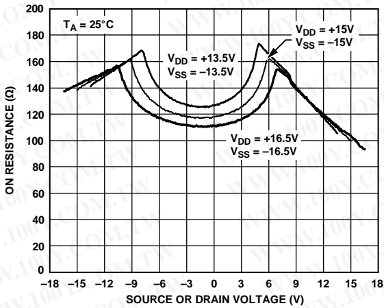
Figure 7. On Resistance as a Function of V_D ( V_S ) for Dual Supply
