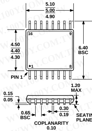
Figure 31. 16-Lead Thin Shrink Small Outline Package [TSSOP] (RU-16)
