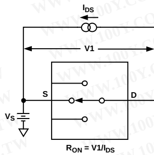
Figure 20. On Resistance
