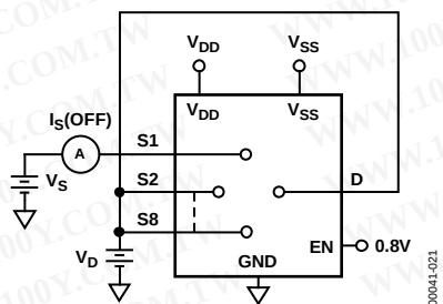
Figure 21. I_S (OFF)
