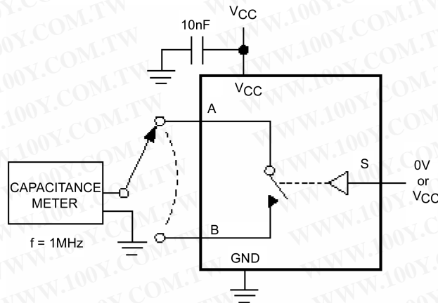
FIGURE 6. ON/OFF Capacitance
