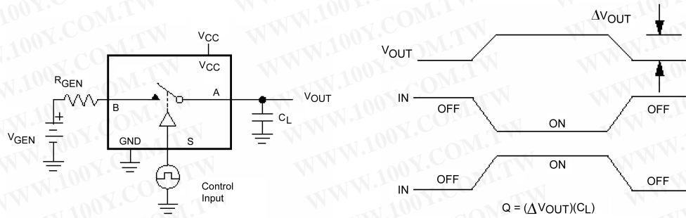
FIGURE 2. Charge Injection
