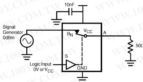
FIGURE 9. Bandwidth
