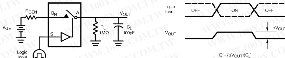
FIGURE 4. Charge Injection Test
