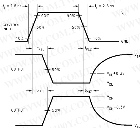
FIGURE 2. AC Waveforms
