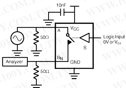
FIGURE 5. Off Isolation
