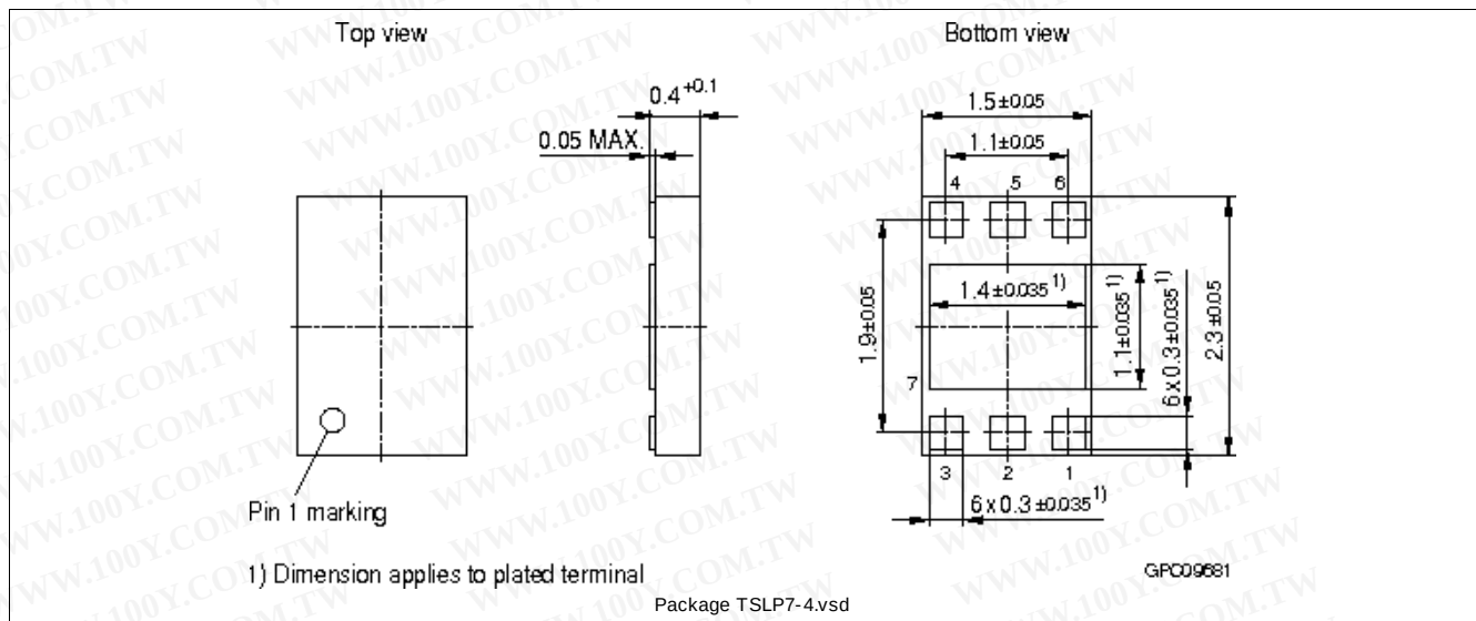
Figure 6 Package TSLP7-4
