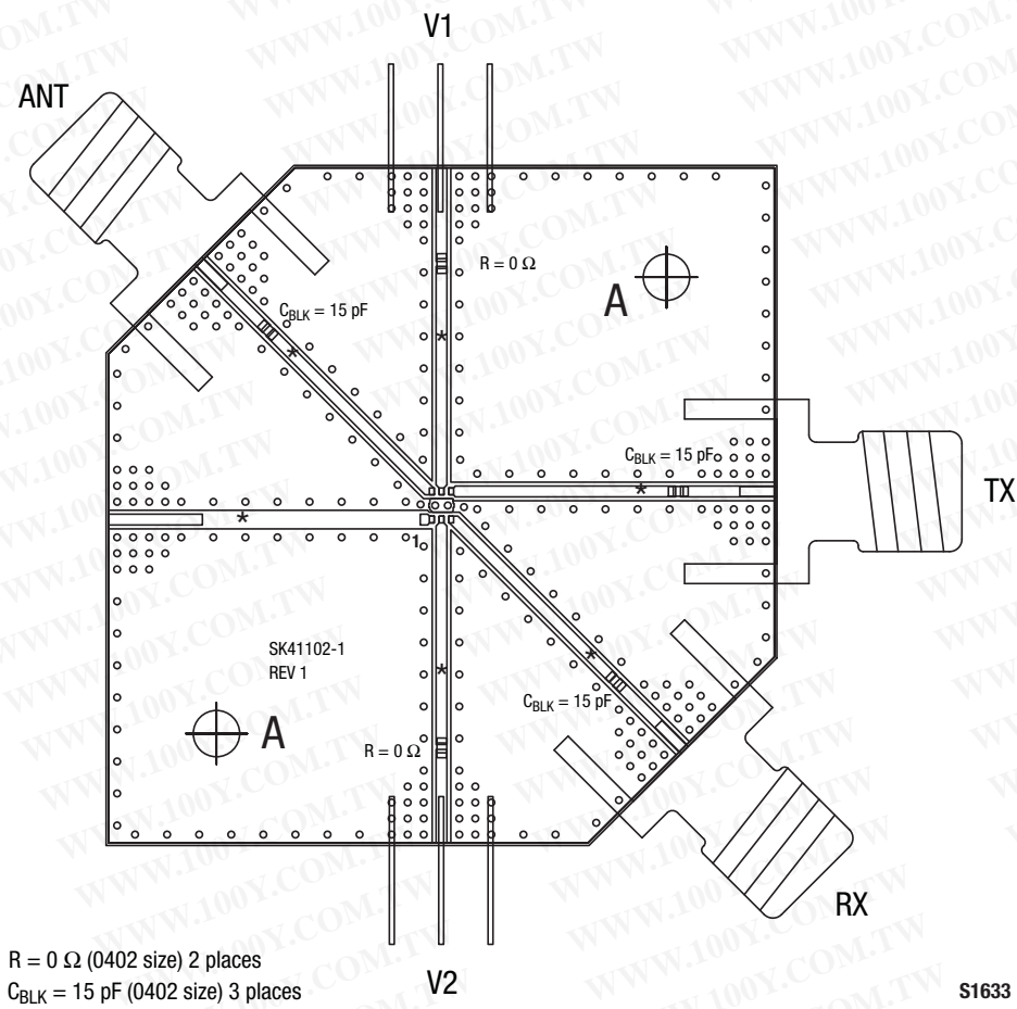
Figure 11. SKY13314-374LF Evaluation Board Assembly Diagram
