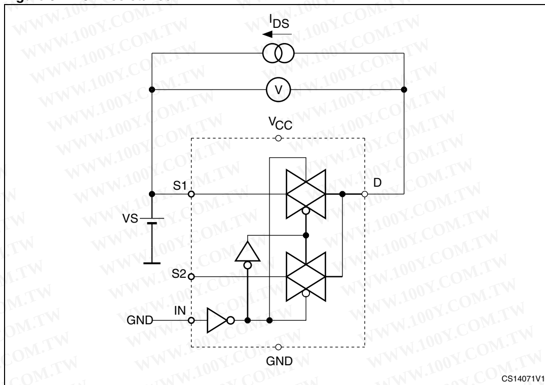
Figure 3. ON-resistance
