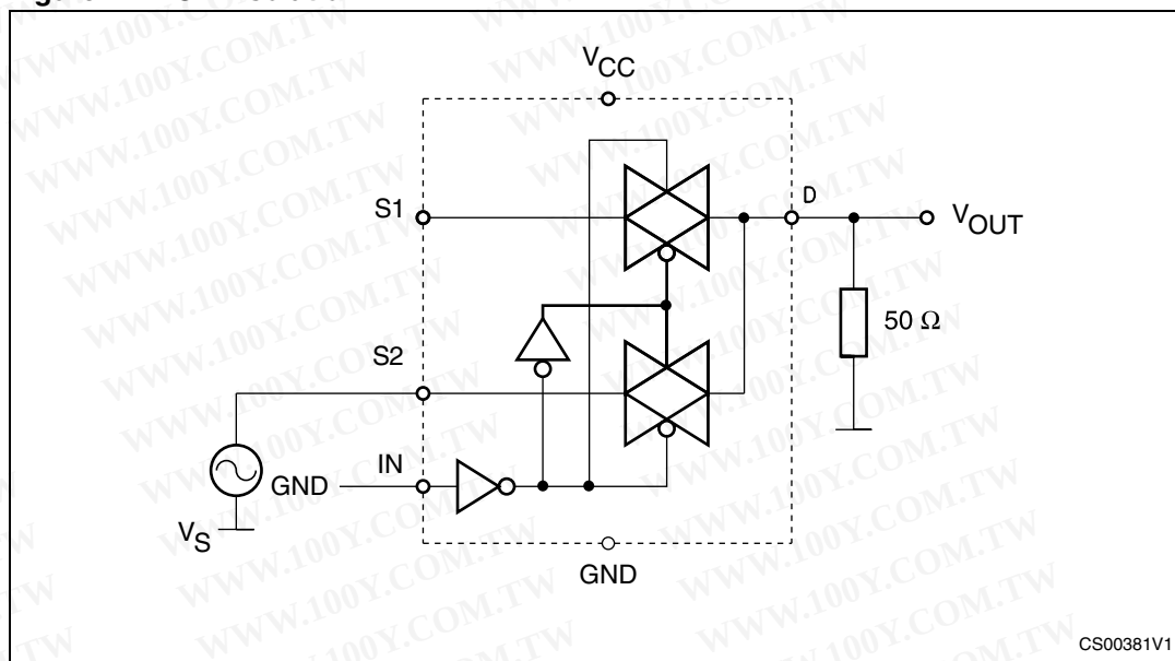
Figure 7. OFF isolation
