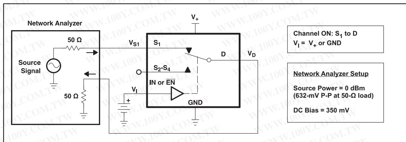
Figure 18. Bandwidth (BW)
