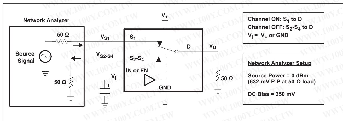
Figure 20. Crosstalk ( X_{TALK} )
