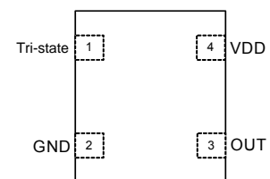
Figure 1. Pin Assignments
