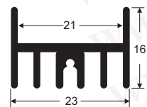
Part No. 1760 Product No. AK-145-25mm 邊孔+pin 說明 金色散熱片 Size 23*25*16mm Part No. 16958 Product No. AK-145-25mm 邊孔 說明 金色散熱片 Size 23*25*16mm Part No. 49435 Product No. AK-145-25mm 邊孔+pin 說明 金色散熱片 Size 23*25*16mm
