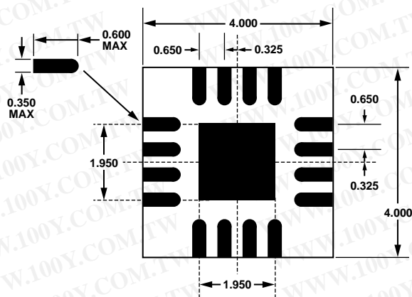
Figure 3. 4 mm × 4 mm 16-pad LFCSP Recommended Pad Layout
