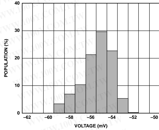
Figure 6. X-Axis Self Test Response at 25°C, V_S = 3 V
