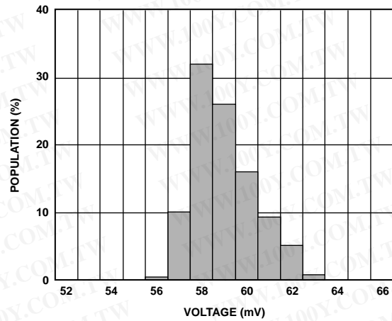
Figure 7. Y-Axis Self Test Response at 25°C, V_S = 3 V
