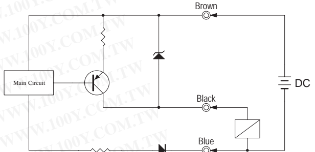
PNP type
