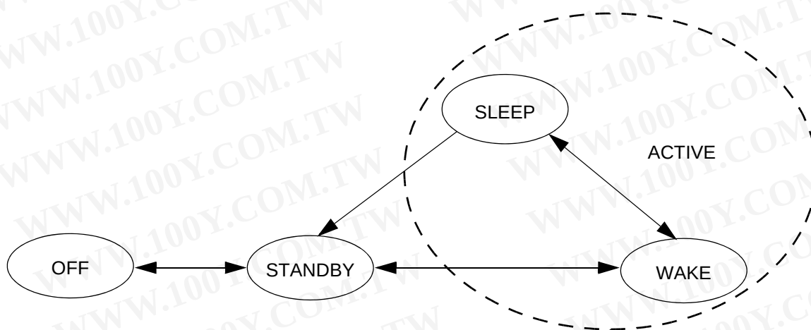
Figure 7. Mode Transition Diagram
