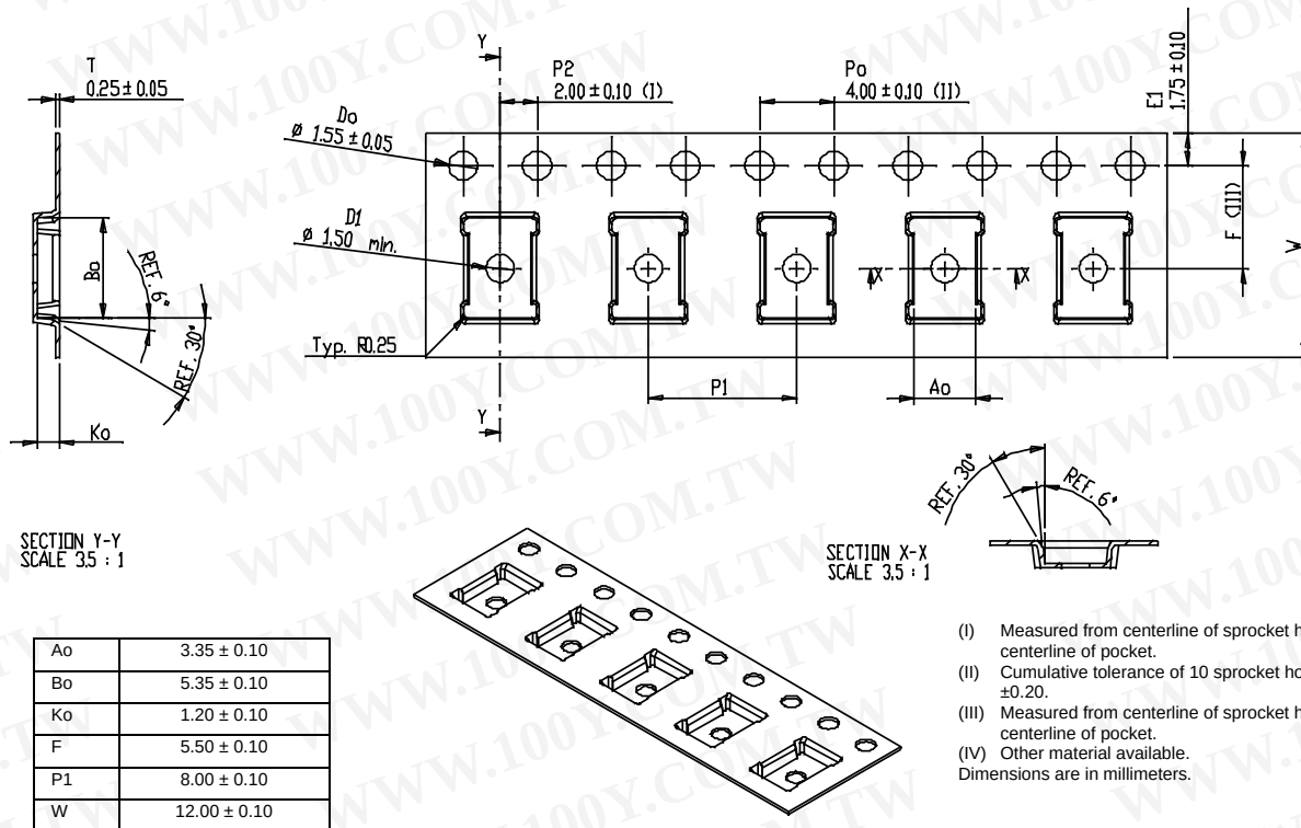
Figure 11. LGA (3 by 5) Embossed Carrier Tape Dimensions
