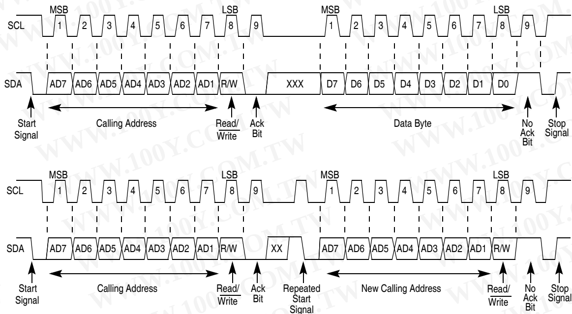
Figure 4. I²C Bus Transmission Signals
