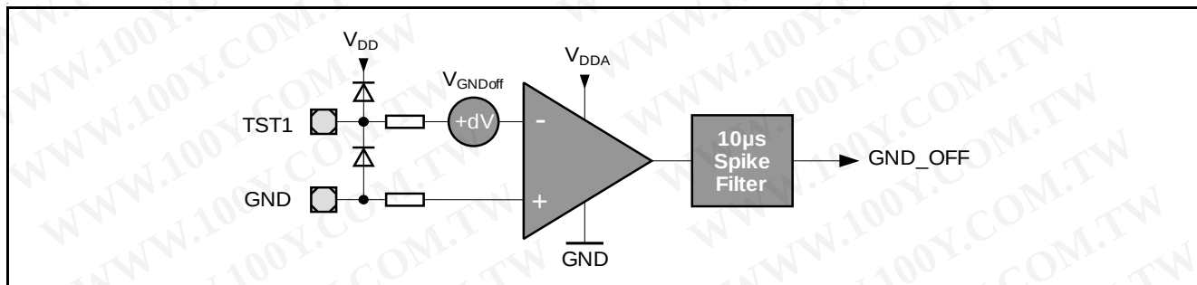
Figure 21 GND-off Comparator
