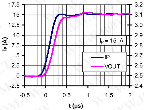
Figure 9: Step response
