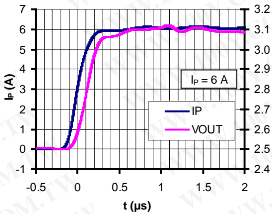
Figure 3: Step response
