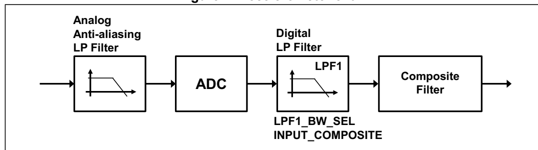
Figure 7. Accelerometer chain
