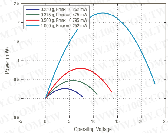
Tuned to 105 Hz | 4.8 gram Tip Mass
