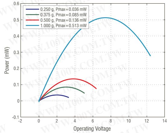
Tuned to 65 Hz | 1 gram Tip Mass
