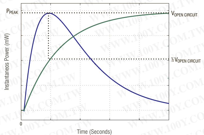
Typical Power & Voltage vs Time
