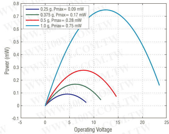
Tuned to 45 Hz | 0.5 gram Tip Mass
