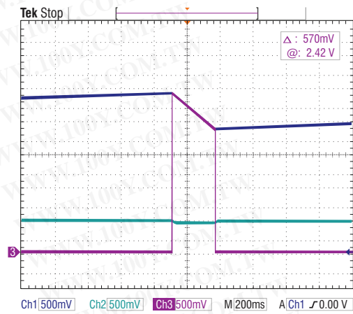
Figure 6: Rectified input (aqua), V_{CAP} (navy) and switched output (violet) output pulse detail, 10K resistive load.
