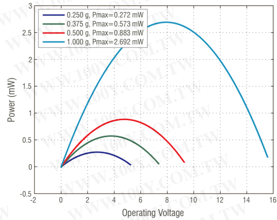
Tuned to 130 Hz | 2.4 gram Tip Mass
