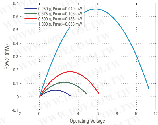
Tuned to 175 Hz | 1 gram Tip Mass
