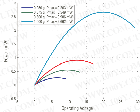
Tuned to 40 Hz | 4.8 gram Tip Mass
