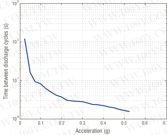
Figure 2: Discharge Interval vs. Acceleration, measured results using configuration shown
