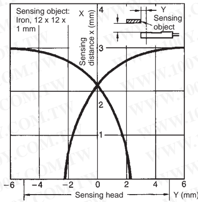
TL-W3M
