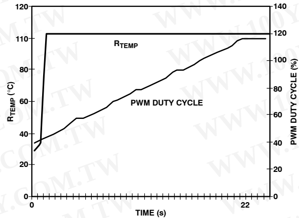
Figure 30. Filtered Mode with Ramp Rate = 4
