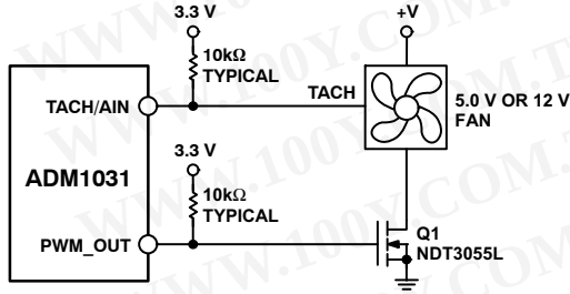
Figure 34. Interfacing the ADM1031 to a 3-Wire Fan
