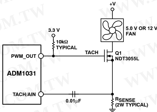
Figure 35. Interfacing the ADM1031 to a 2-Wire Fan
