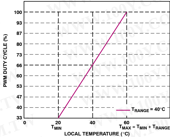
Figure 24. Maximum Speed Calculated by Local Temperature Control Loop Drives Fan
