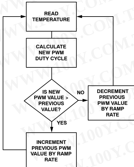
Figure 28. Filtered Mode Algorithm
