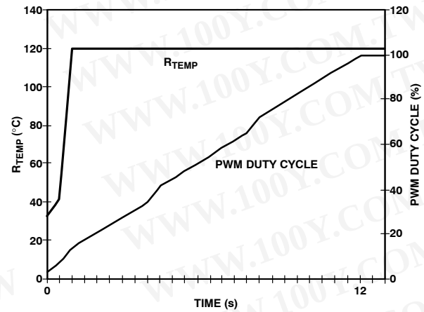
Figure 29. Filtered Mode with Ramp Rate = 8
