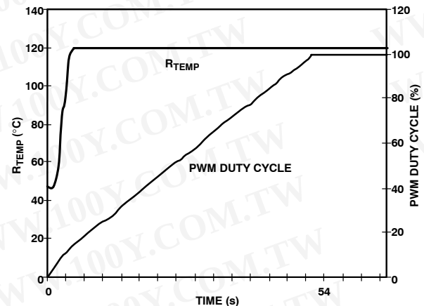
Figure 31. Filtered Mode with Ramp Rate = 2
