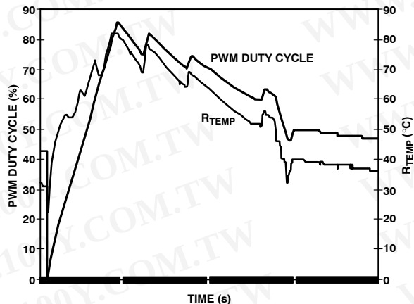
Figure 33. How Fan Reacts to Temperature Variation in Filtered Mode
