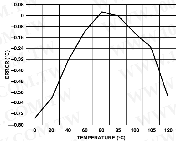
Figure 12. Remote Temperature Sensor Error
