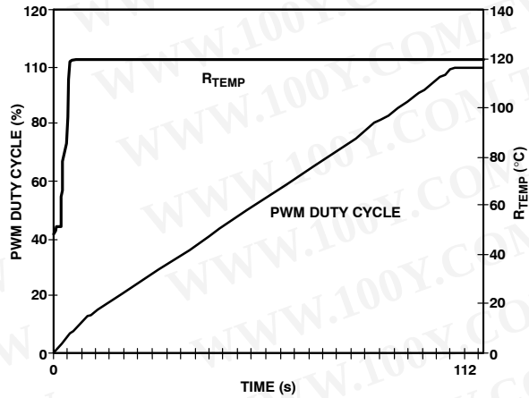
Figure 32. Filtered Mode with Ramp Rate = 1
