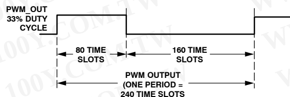
Figure 27. 33% PWM Duty Cycle Presented in Time Slots
