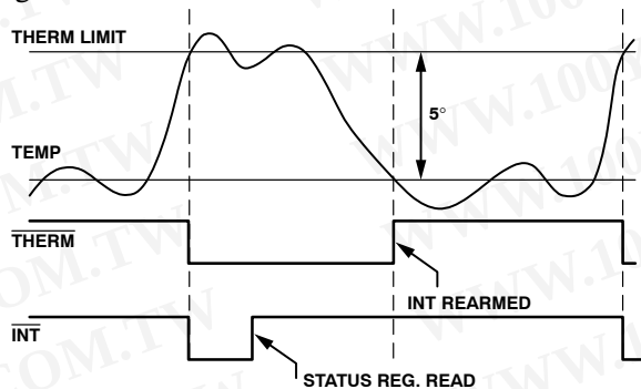
Figure 20. Operation of THERM and INT Signals
