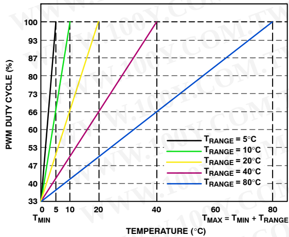
Figure 22. PWM Duty Cycle vs. Temperature Slope ( T_{\text{RANGE}} )
