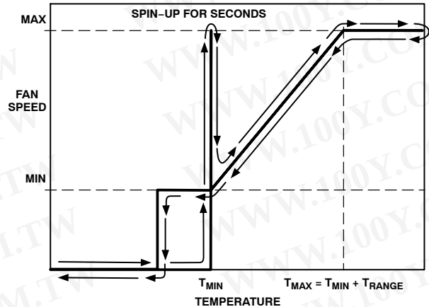
Figure 21. Automatic Fan Speed Control Loop
