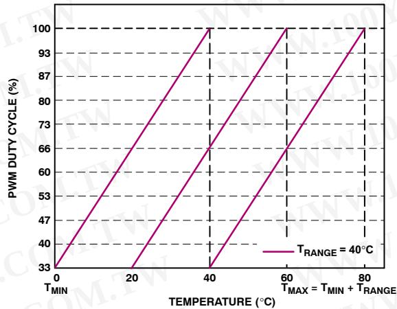
Figure 23. Effect of Increasing T_{\text{MIN}} Value on Control Loop
