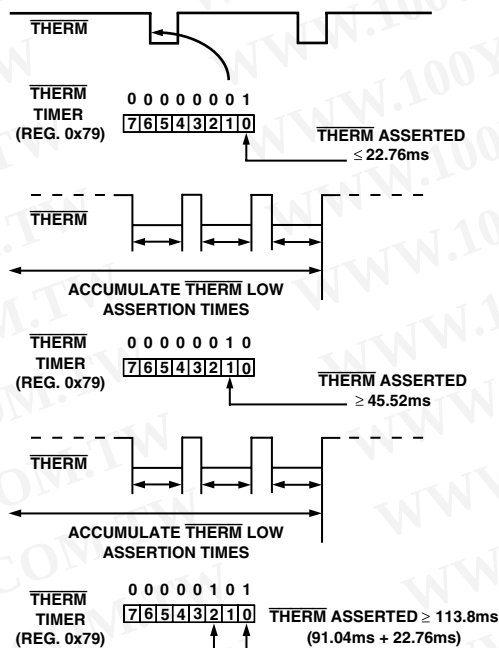
Figure 26. Understanding the THERM Timer
