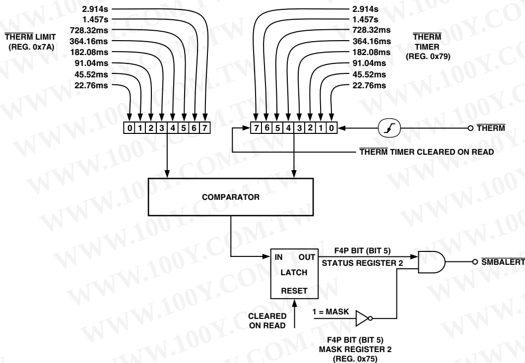
Figure 27. Functional Diagram of ADT7463's THERM Monitoring Circuitry
