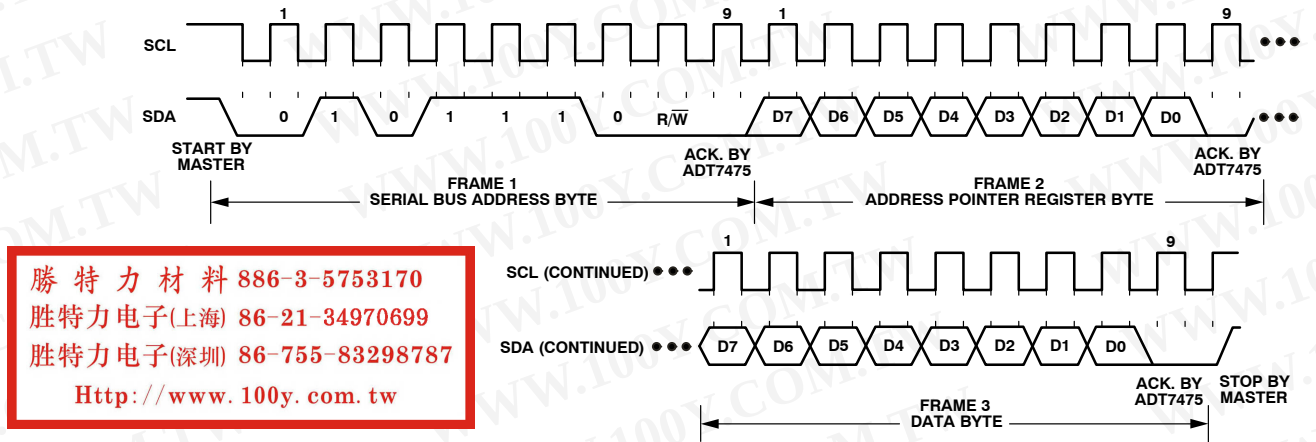
Figure 13. Writing a Register Address to the Address Pointer Register, then Writing Data to the Selected Register
