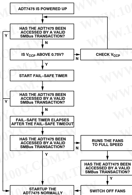
Figure 41. Power-On Flow Chart
