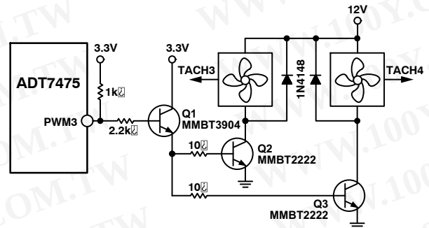
Figure 33. Interfacing Two Fans in Parallel to the PWM3 Output Using Low Cost NPN Transistors
