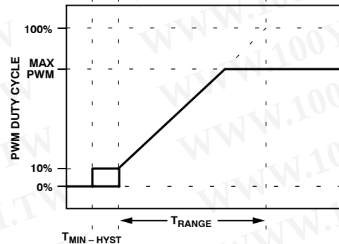
Figure 55. Changing \text{PWM}_{\text{MAX}} Does Not Change the AFC Slope
