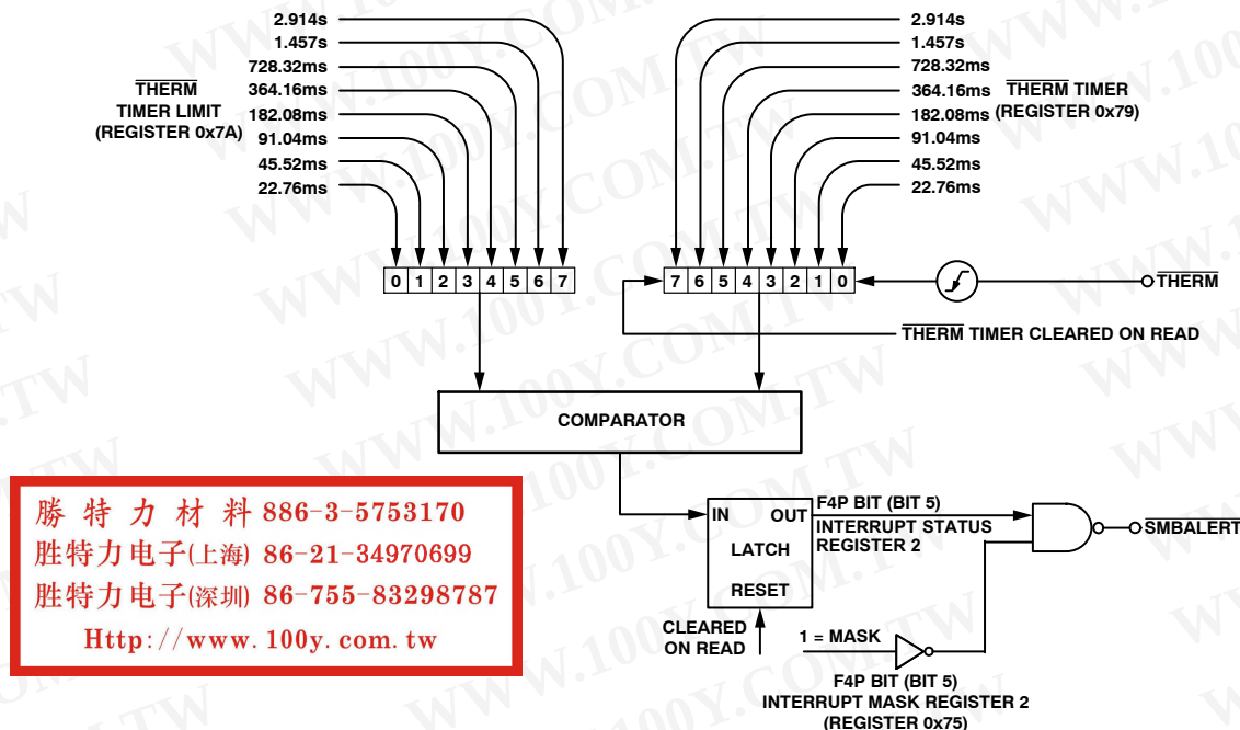
Figure 28. Functional Block Diagram of the ADT7475 THERM Monitoring Circuitry
