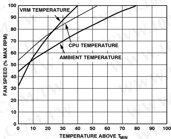
Figure 58. T_{RANGE} and % Fan Speed Slopes for VRM, Ambient, and CPU Temperature Channels
