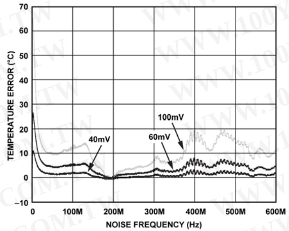
Figure 6. Remote Temperature Error vs. Differential Mode Noise Frequency
