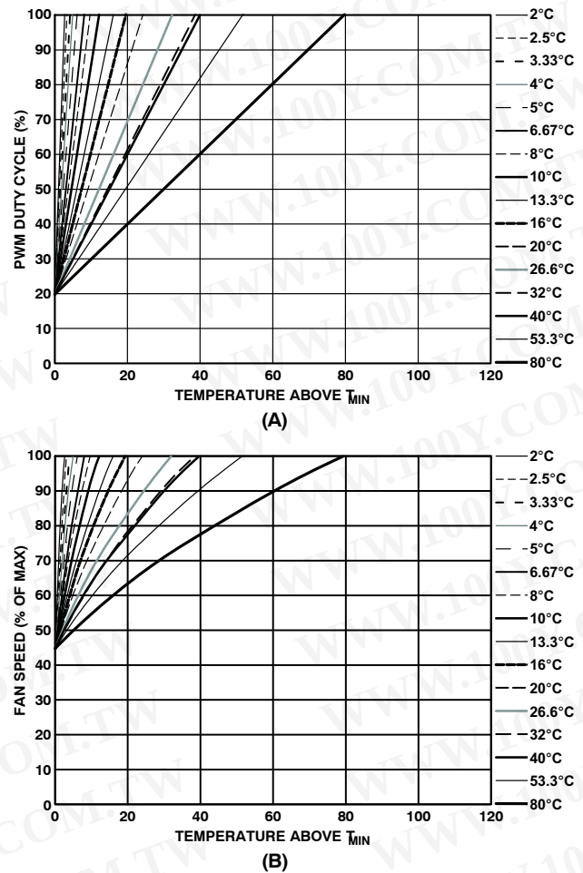
Figure 57. T_{\text{RANGE}} and % Fan Speed Slopes with \text{PWM}_{\text{MIN}} = 20\%
