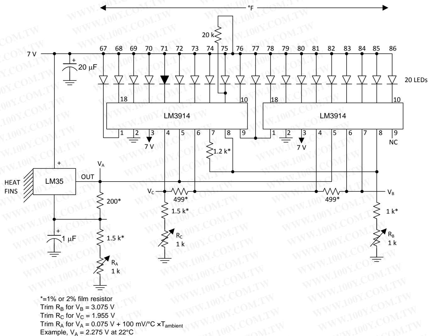
Figure 26. Bar-Graph Temperature Display (Dot Mode)
