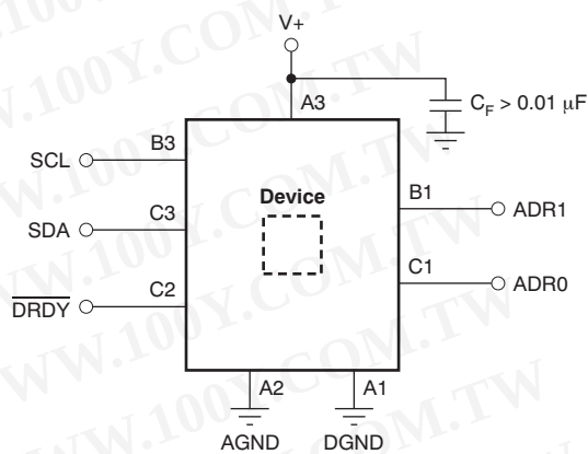
Figure 4. Typical Connection Diagram
