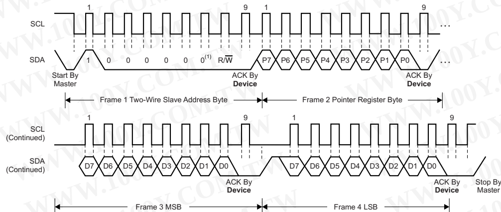
Figure 7. Two-Wire Timing Diagram for Write Word Format
