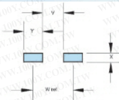
Land Pattern
