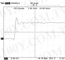
Expand (10nsec/div, 2V/div)
