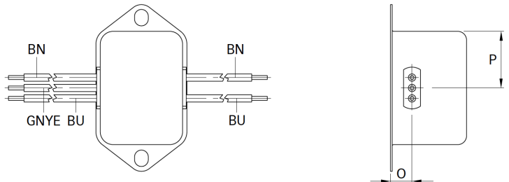
Connection style -07, 1 A types (same dimensions as style -06)
