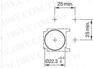
Mounting cut-outs [mm]
