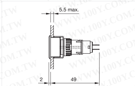
Dimensions [mm]
