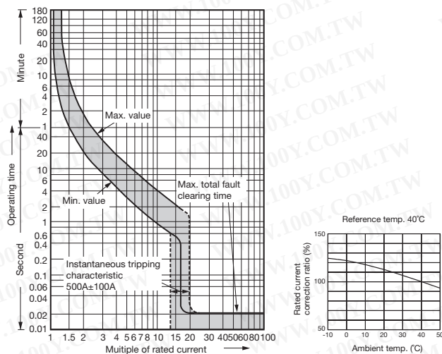
● BW125, EW125 (Rated current: 50 - 125A)
