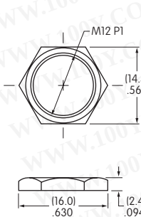
AT503M Hex Face Nut Brass/Chrome
