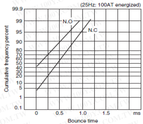
(2) Bounce time
