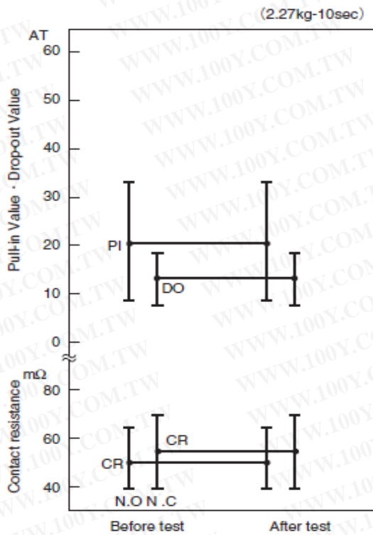
(1) Lead tensile test (static load)
