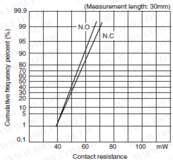
(2) Contact resistance
