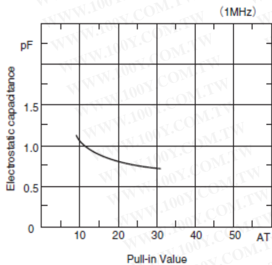
(5) Electrostatic capacitance
