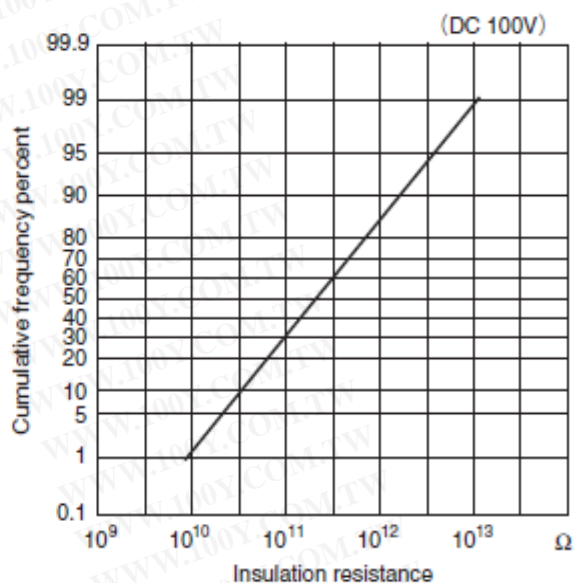
(4) Insulation resistance
