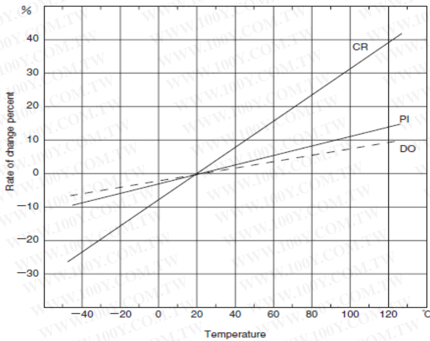
(1) Temperature characteristics
