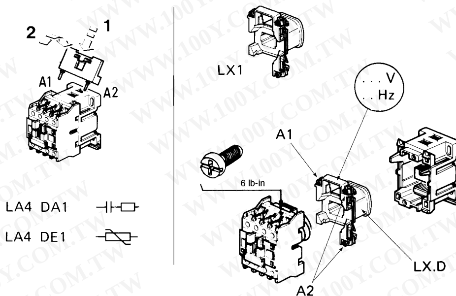
Figure 3 Mounting Interface Modules, Top Mounted Contact Block and Coil Suppressor to Contactors / Coil Replacement
