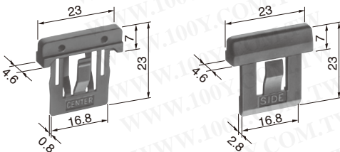
Center Barrier for Guard Cover
