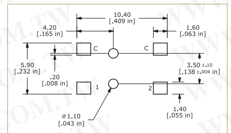
P.C. MOUNTING
