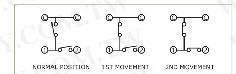
SCHEMATIC
