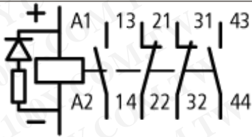
DC Coil
