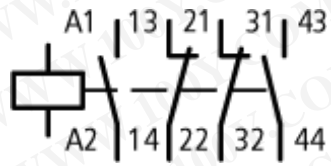
AC Coil
