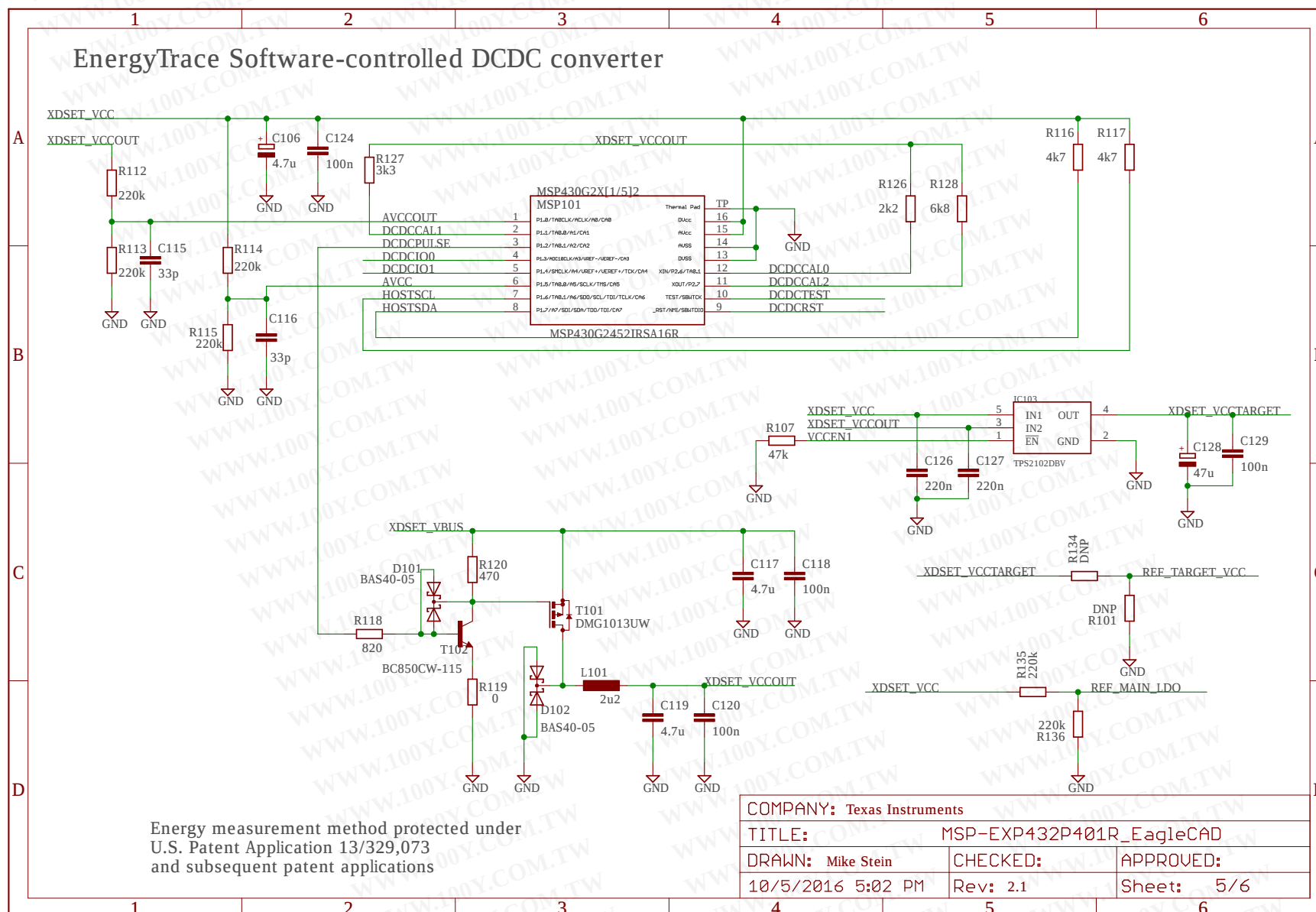
Figure 32. Schematics (5 of 6)
