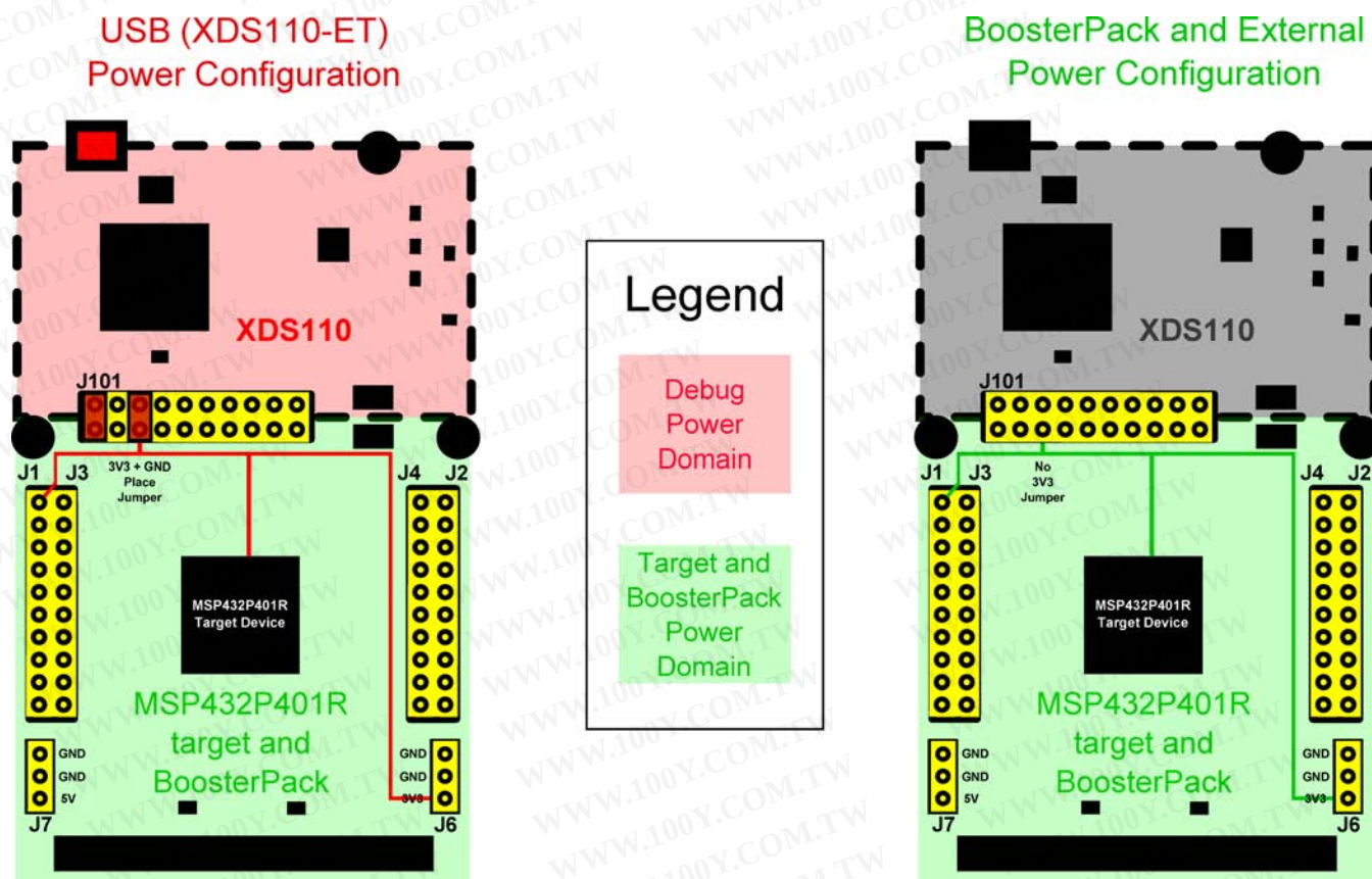
Figure 10. MSP-EXP432P401R Power Block Diagram
