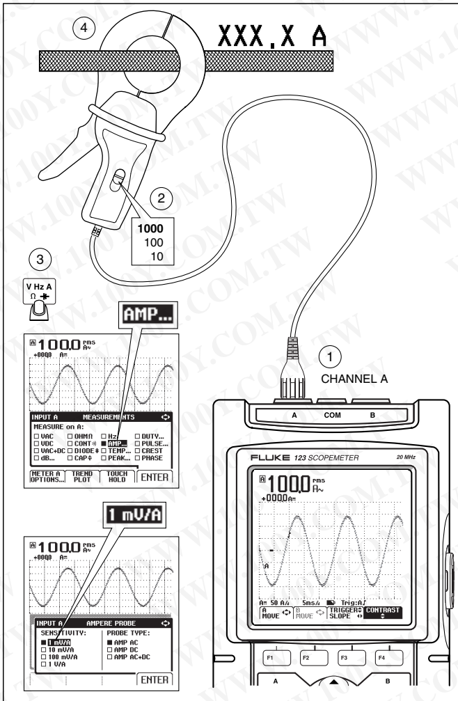
Figure 3. ScopeMeter Setups
