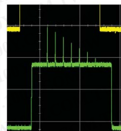
DDS at 50 kHz
