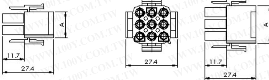
9, 12, 15 Circuit (Matrix)
