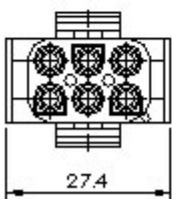
6 Circuit (Matrix)
