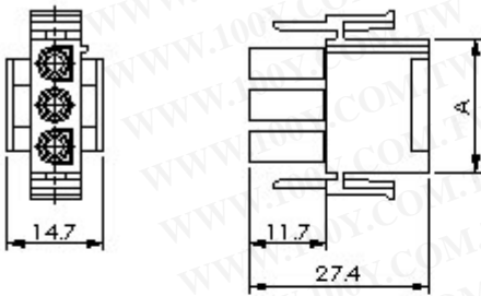
2, 3, 4 Circuit (h-Line)
