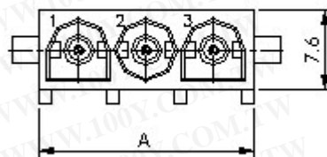
2, 3, 4 Circuit (In-Line)
