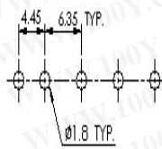
PC Board Layout
