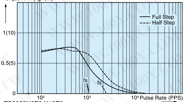
TS3653N2E6,N12E6 Torque N·m (kgf·cm)
