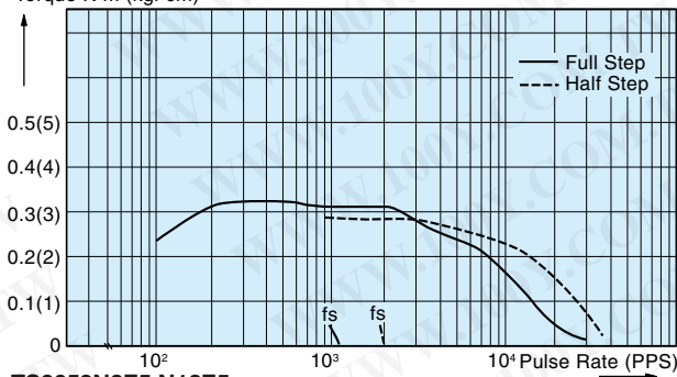
TS3653N2E5,N12E5 Torque N·m (kgf·cm)
