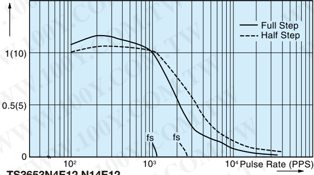
TS3653N4E12,N14E12 Torque N·m (kgf·cm)
