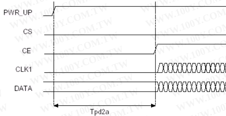
Figure 9 VDD off to active mode
