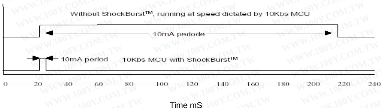
Figure1 Current consumption with & without ShockBurst™ technology
