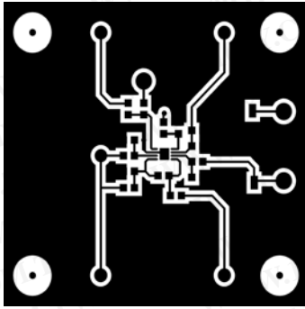
Figure 9. Dual-Supply Component Side Copper
