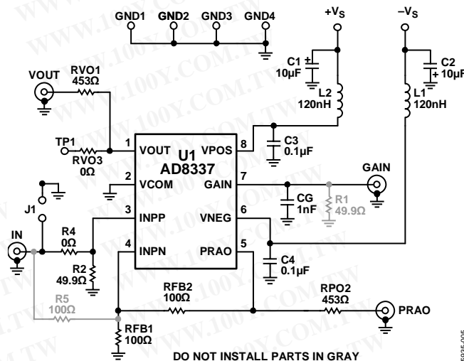
Figure 5. Evaluation Board Schematic—Noninverting Configuration
