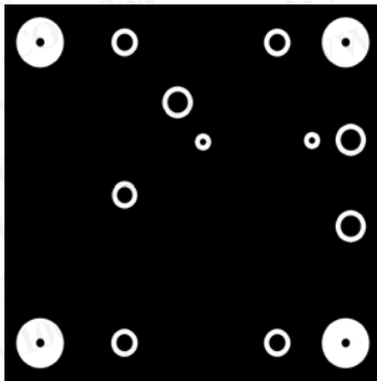
Figure 10. Dual-Supply Wiring Side Copper
