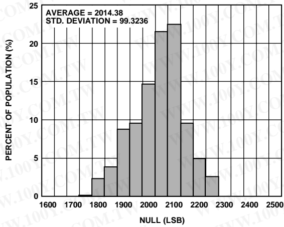
Figure 6. Initial Null Histogram
