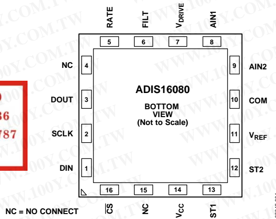
Figure 4. Pin Configuration
