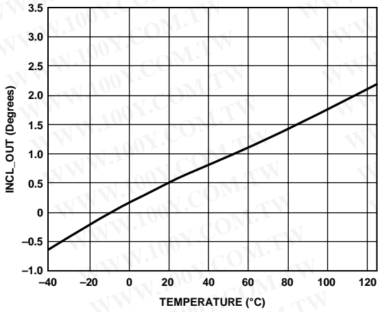
Figure 6. Inclination Error vs. Temperature
