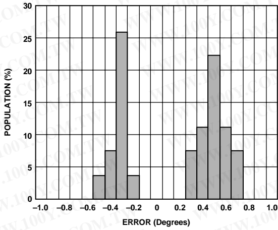
Figure 5. Inclination Error Distribution at 25°C/3.3 V, Incline = 0°
