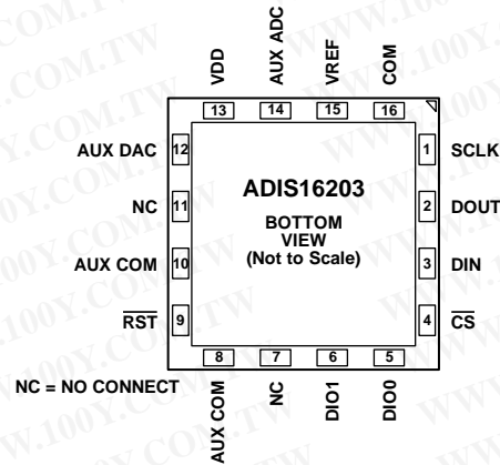
Figure 4. Pin Configuration
