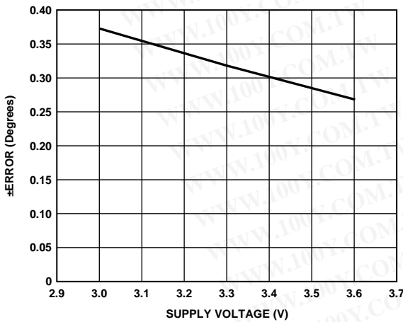
Figure 7. Inclination Error vs. Supply
